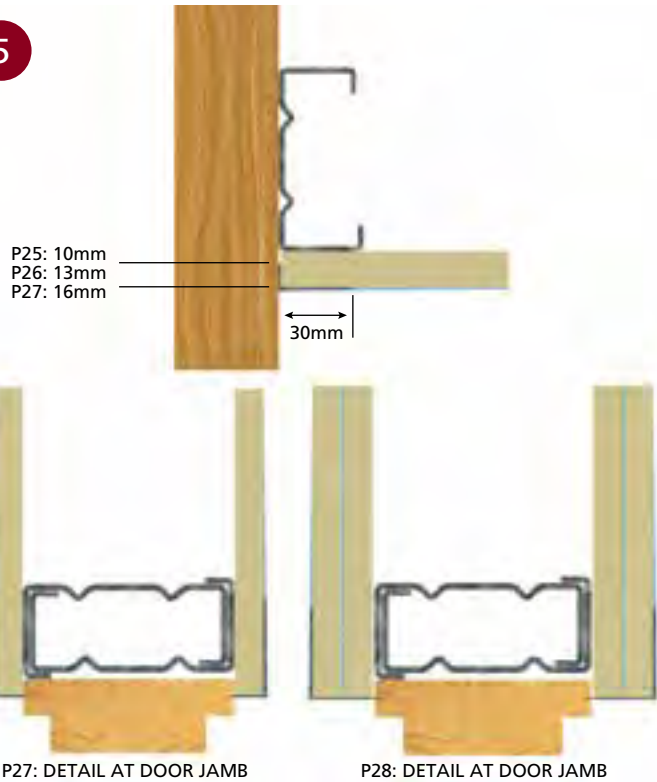
P27: DETAIL AT DOOR JAMB
