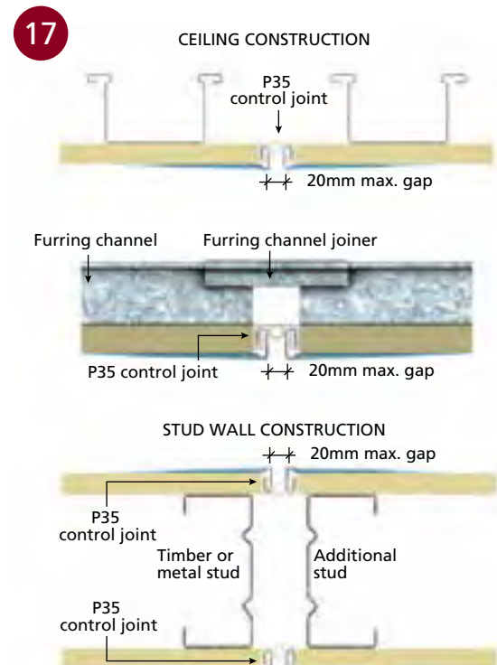
■ P35 INSTALLATION
